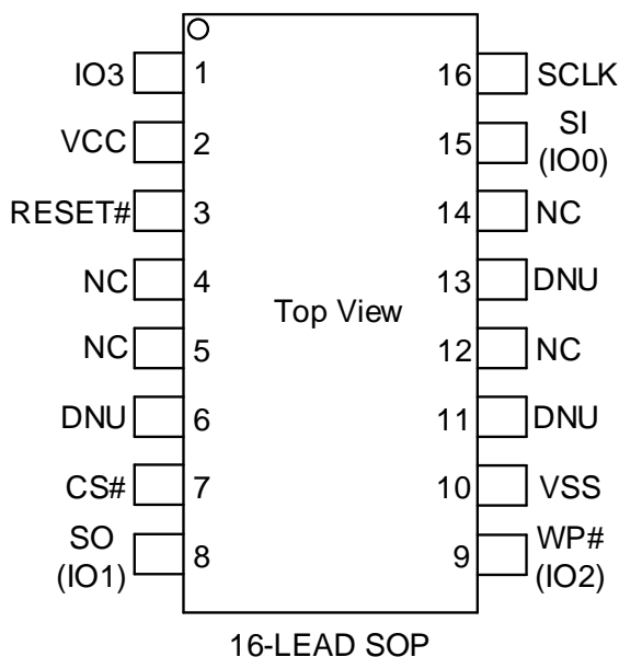
Figure 2 Connection Diagram for SOP16 package
