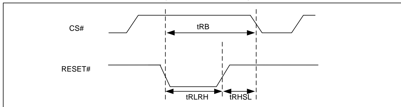
Figure 102. RESET Timing
