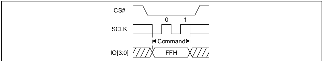
Figure 60 Disable QPI mode command Sequence Diagram
