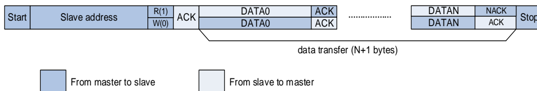
Figure 20-7. I2C communication flow with 10-bit address (Master Transmit)
