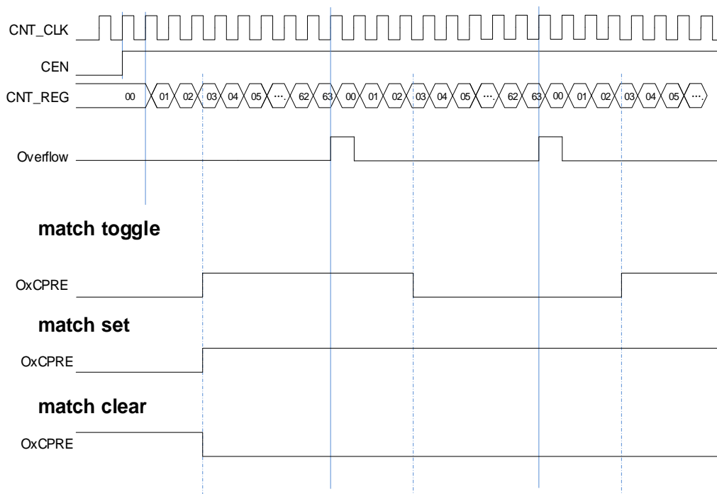
Figure 18-13. Output-compare under three modes
