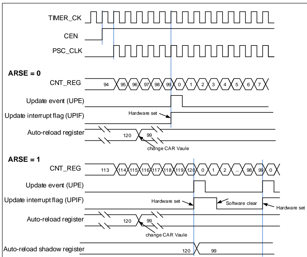
Figure 18-60. Timing chart of up counting mode, change TIMEx_CAR ongoing
