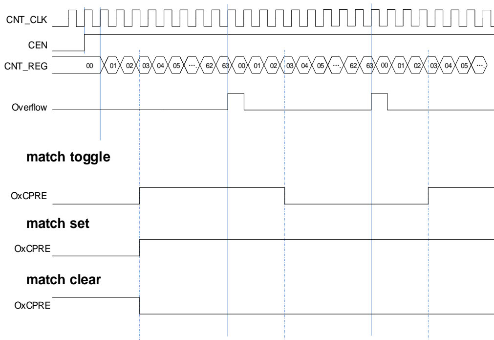
Figure 18-62. Output-compare under three modes
