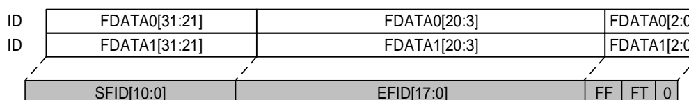
Figure 26-9. 32-bit list mode filter
