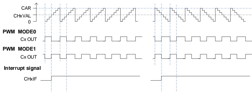
Figure 18-15. CAPWM timechart
