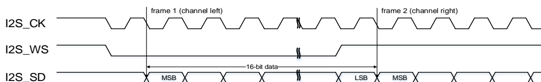
Figure 21-15. I2S Philips standard timing diagram (DTLEN=00, CHLEN=0, CKPL=1)
