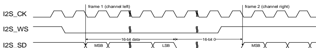
Figure 21-20. I2S Philips standard timing diagram (DTLEN=00, CHLEN=1, CKPL=0)
