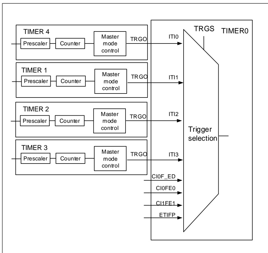
Figure 18-26. Timer0 master/slave mode timer example
