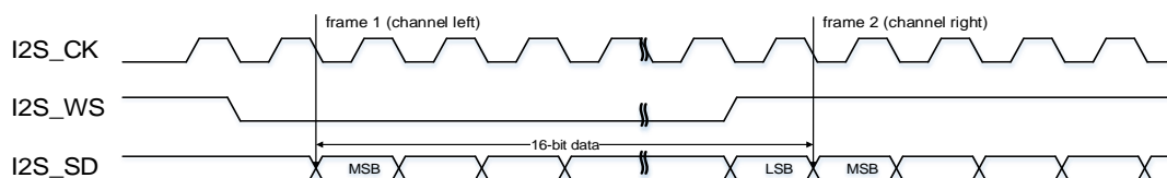
Figure 21-14. I2S Philips standard timing diagram (DTLEN=00, CHLEN=0, CKPL=0)
